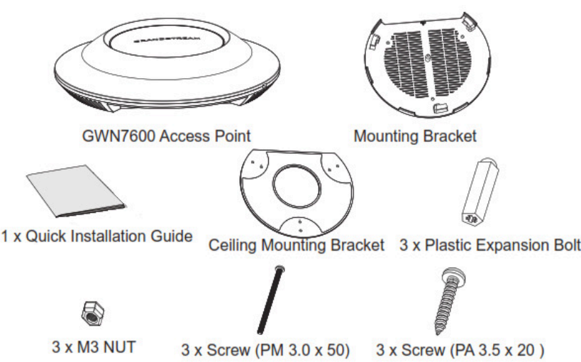
GWN76xx Equipment Packaging
