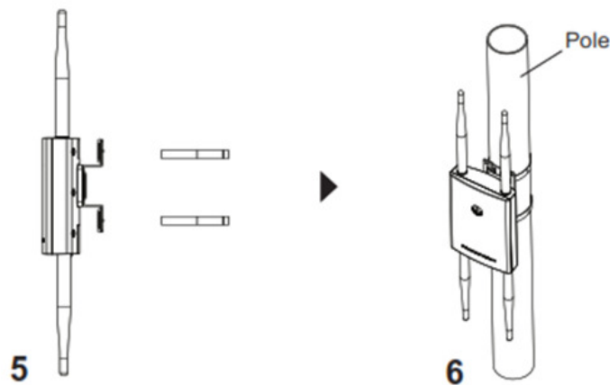
GWN7630LR/GWN7605LR/GWN7660LR /GWN7664LR Pole Mount
