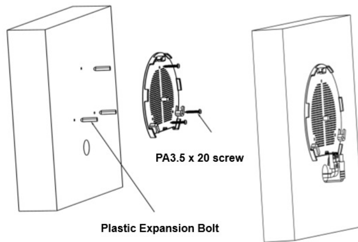
Wall Mount – Steps 3 & 4
