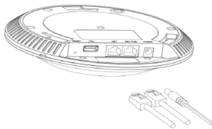
Connecting GWN AP – GWN7600 as an example
