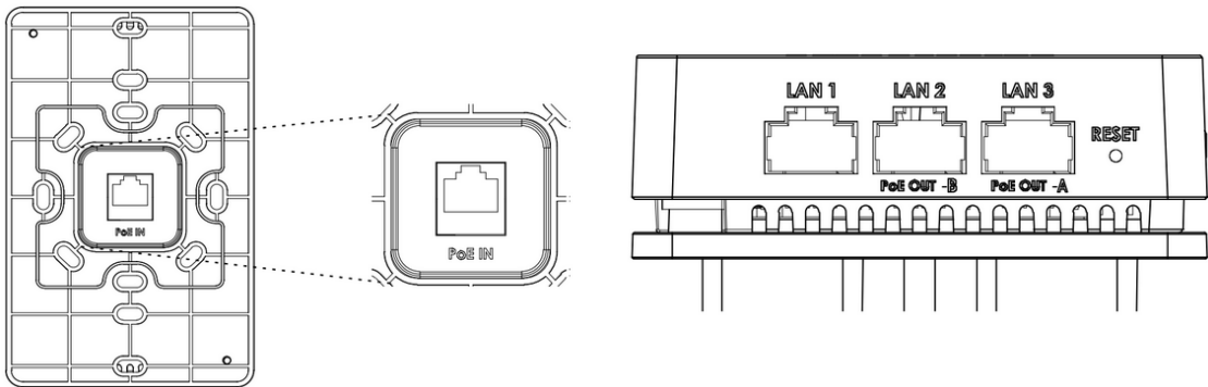
GWN7624/GWN7661/GWN7661E Ports
