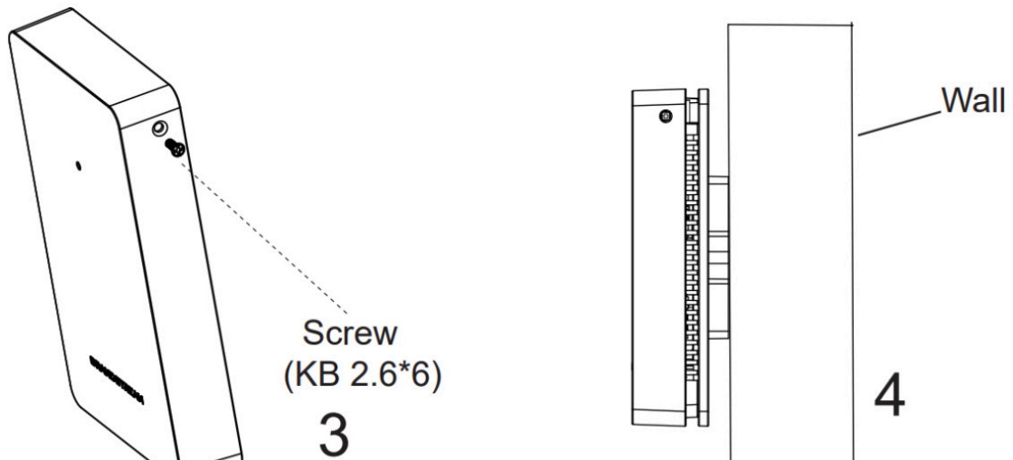
GWN7624/GWN7661/GWN7661E Wall Installation
