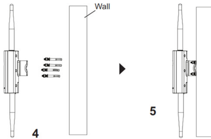
GWN7630LR/GWN7605LR/GWN7660LR Wall Mount
