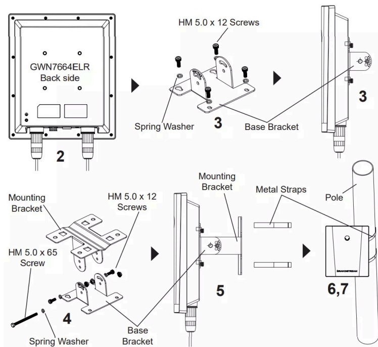
Pole Mount
