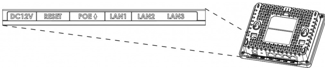
GWN7602/GWN7603/GWN7604 Ports
