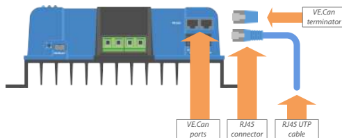
VE.Can port, connector, terminator and cable
