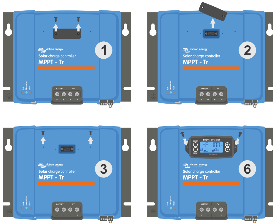
How and where to connect the SmartSolar Control display
