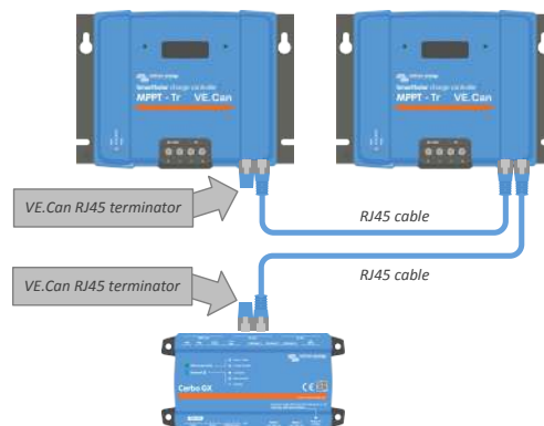
Example of two VE.Can solar chargers connecting to a single GX device
