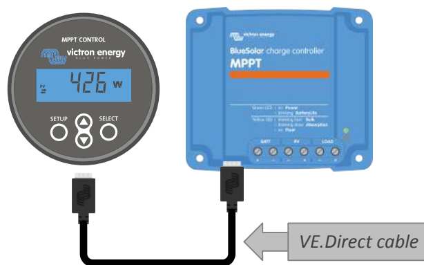
Connect the display to the solar charger via a VE.Direct cable
